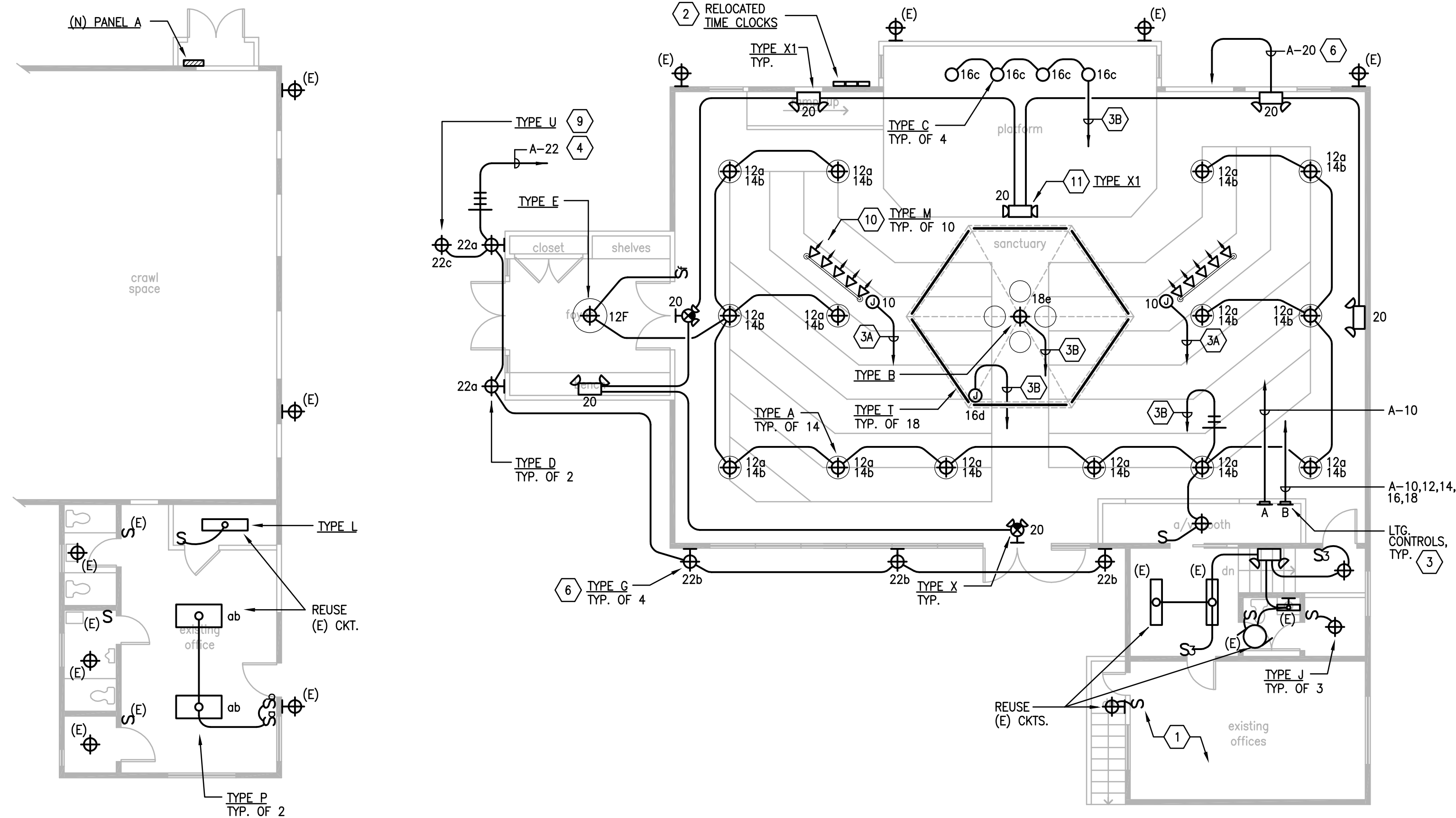
1 NEW LIGHTING PLAN LOWER LEVEL SANCTUARY SCALE: 1/8" = 1'-0"
