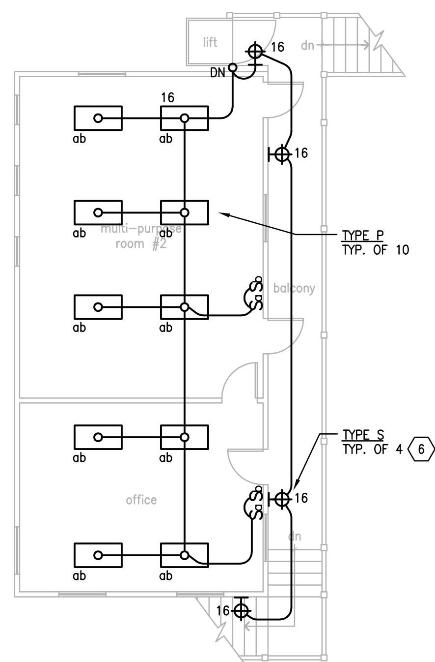
4 NEW LIGHTING PLAN 2ND FLOOR YOUTH EDUCATION BLDG. SCALE: 1/8" = 1'-0"
