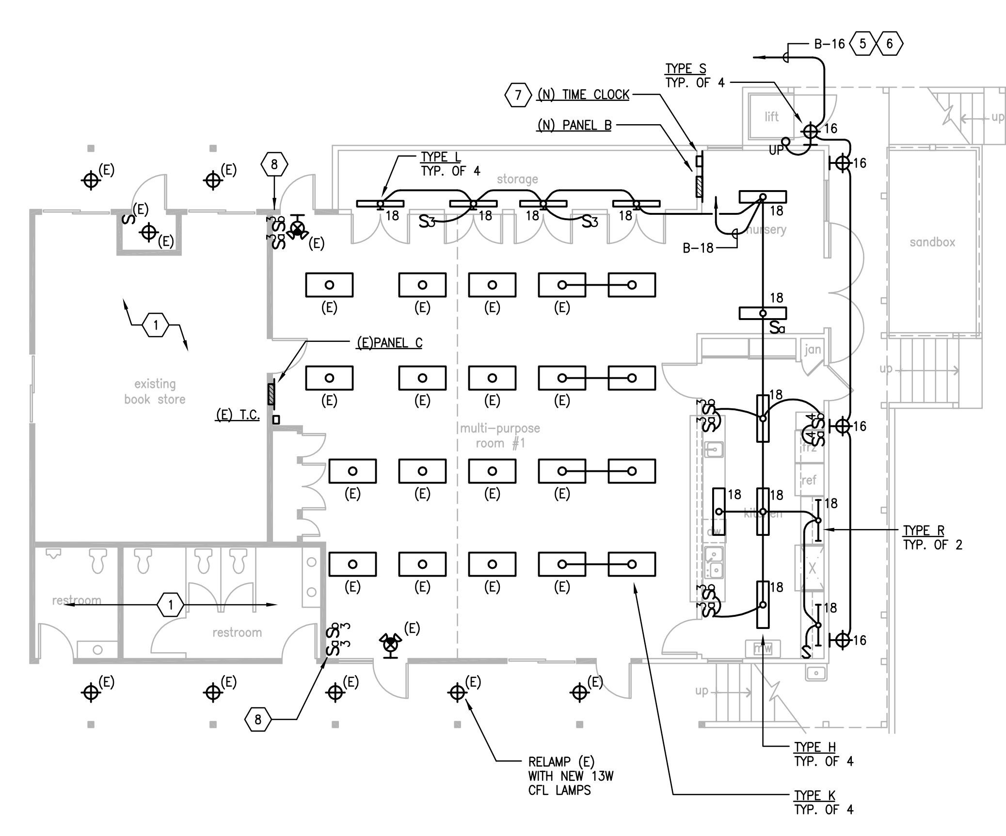
3 NEW LIGHTING PLAN 1ST FLOOR YOUTH EDUCATION BUILDING SCALE: 1/8" = 1'-0"
